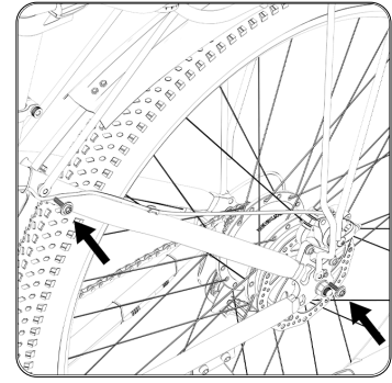
12. Tighten the rear shelf screws.
